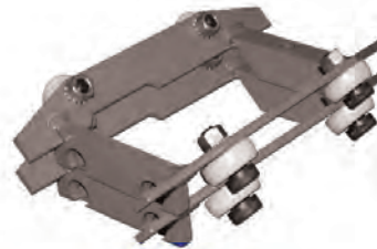
Mainline Skid Assy w/Wheels:
